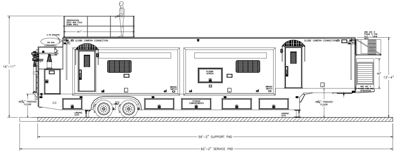
Figure 2: Right Side Elevation
