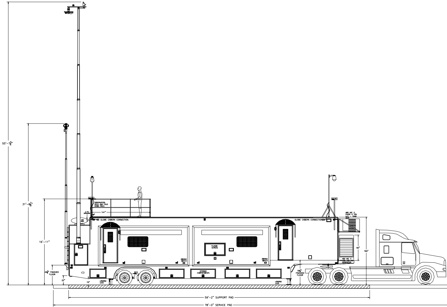
Figure 6: Right Side Elevation with Tractor
