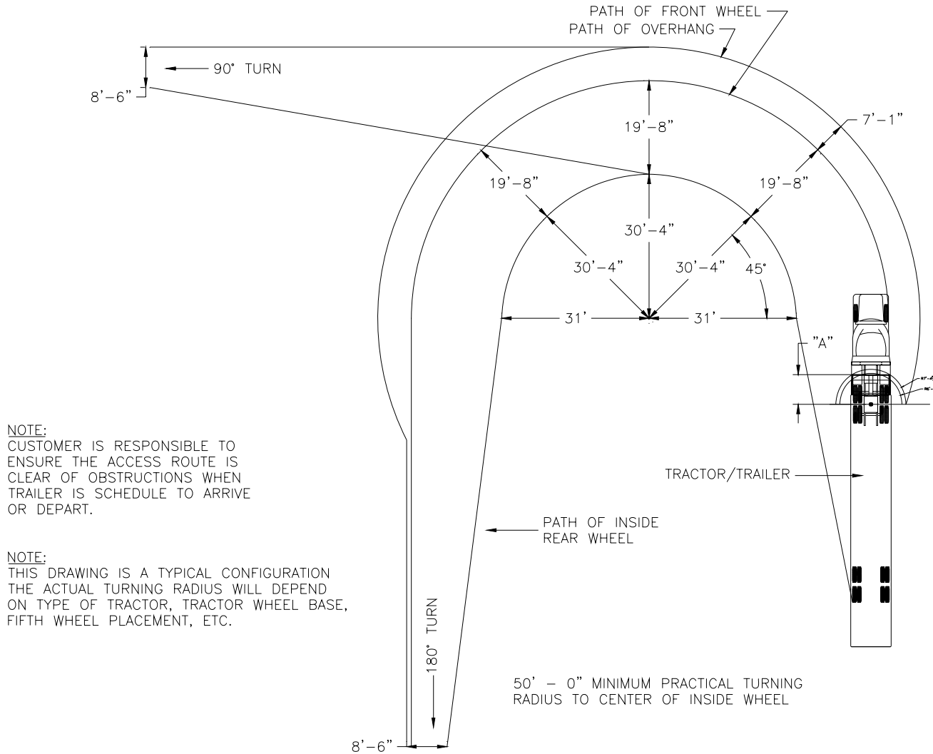
Figure 5: Turning Requirements
