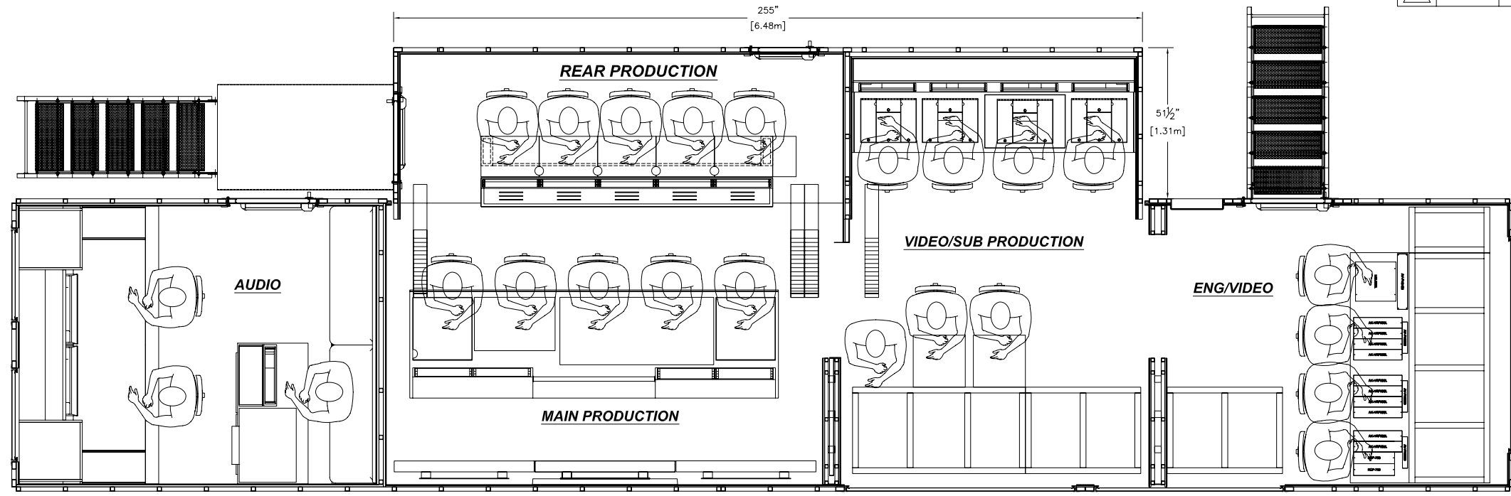
PLAN VIEW
